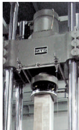
Compression Platens
